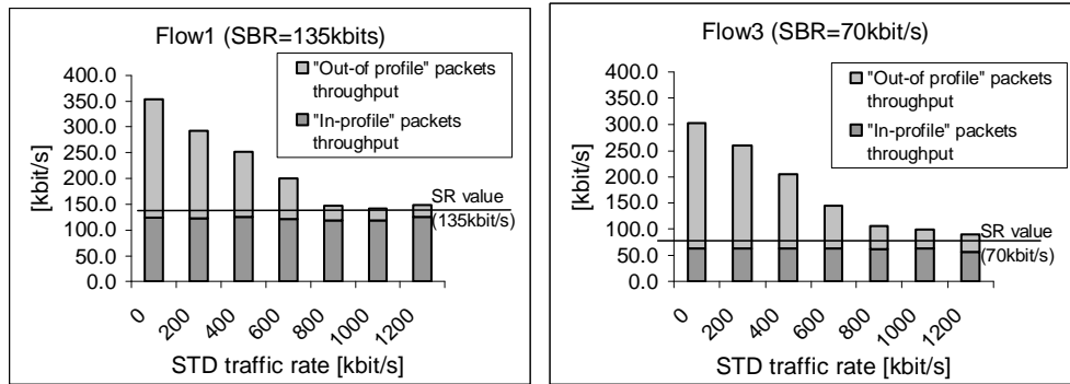
Figure 11 Throughput of “in-profile” and “out-of-profile” packet streams within flow 1 and flow3.
