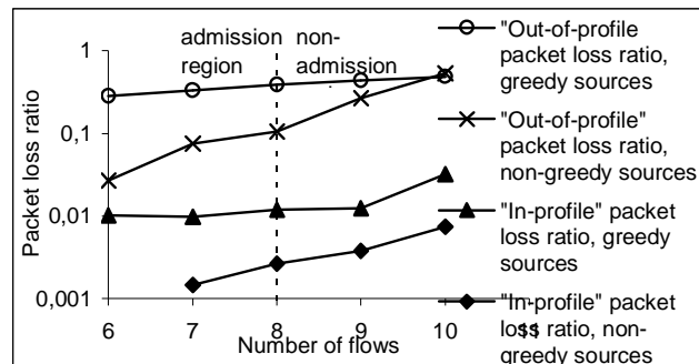
Figure 13 “In-profile” and “Out-of-profile” packet loss ratio vs. number of greedy and non-greedy TCP flows in PMC service.
