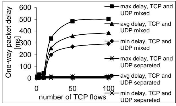
Figure 5 One-way delay of UDP packets mixed with TCP traffic and separated from TCP traffic.
