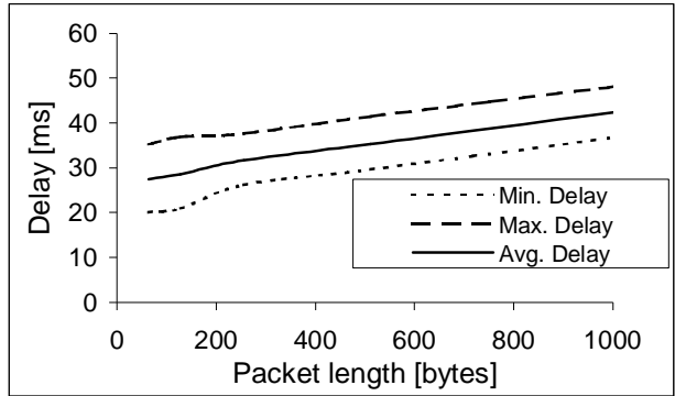
Figure 8 One-way delay vs. TCL 1 packet length.
