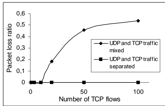
Figure 6 Packet loss ratio of UDP packets mixed with TCP traffic and separated from TCP traffic.
