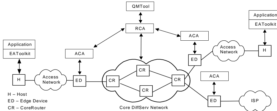
Figure 1 General AQUILA Network Architecture.
