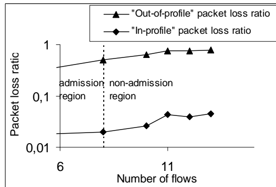
Figure 12 “In-profile” and “out-of-profile” packet loss ratio vs. number of TCP flows in PMM service.
