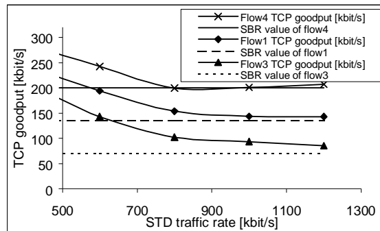
Figure 10 TCP goodput in PMM service vs. STD traffic rate.
