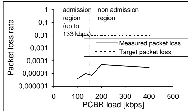
Figure 7 Packet loss rate vs. TCL 1 traffic load.
