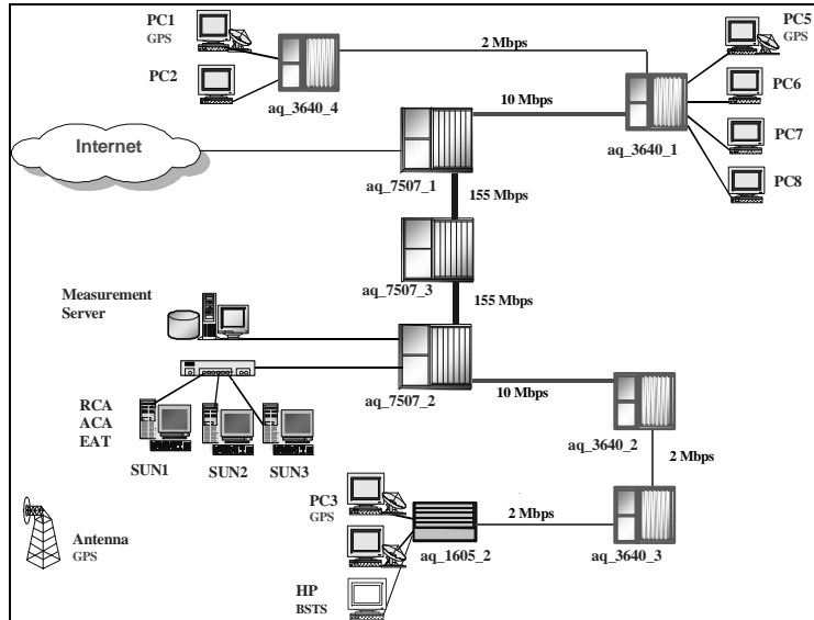
Figure 4 AQUILA test-bed configuration. PC1-8 – terminals, SUN1-3 – SUN Work Stations with implemented RCA, ACA and EAT modules, aq_1605, aq_3640, aq_7507 – CISCO routers.
