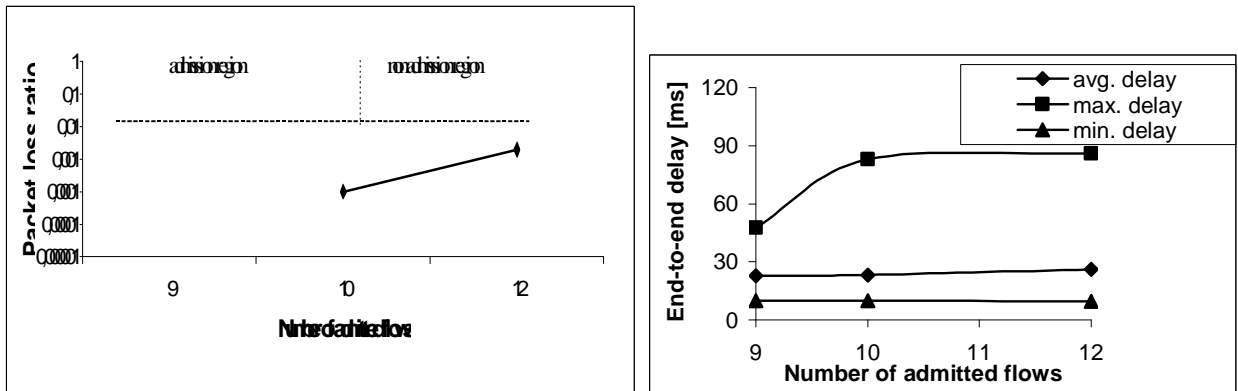
Figure 9 Packet loss ratio vs. number of admitted flows.
