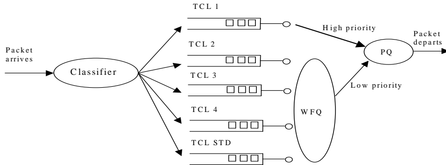
Figure 2 Routers output port architecture.
